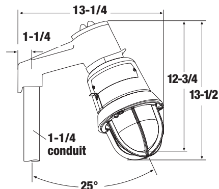
Stanchion mount
